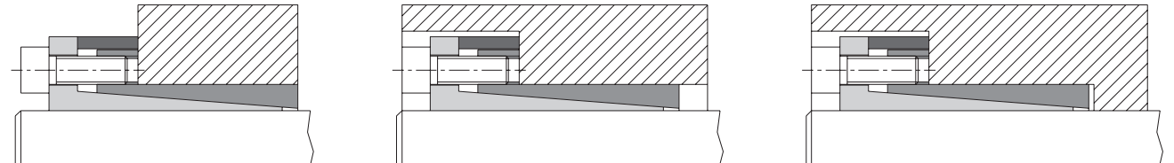
Example of application of hub design
